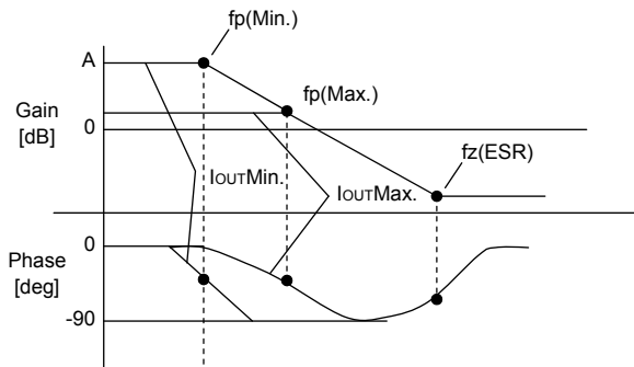
Fig.30 Open loop gain characteristics
